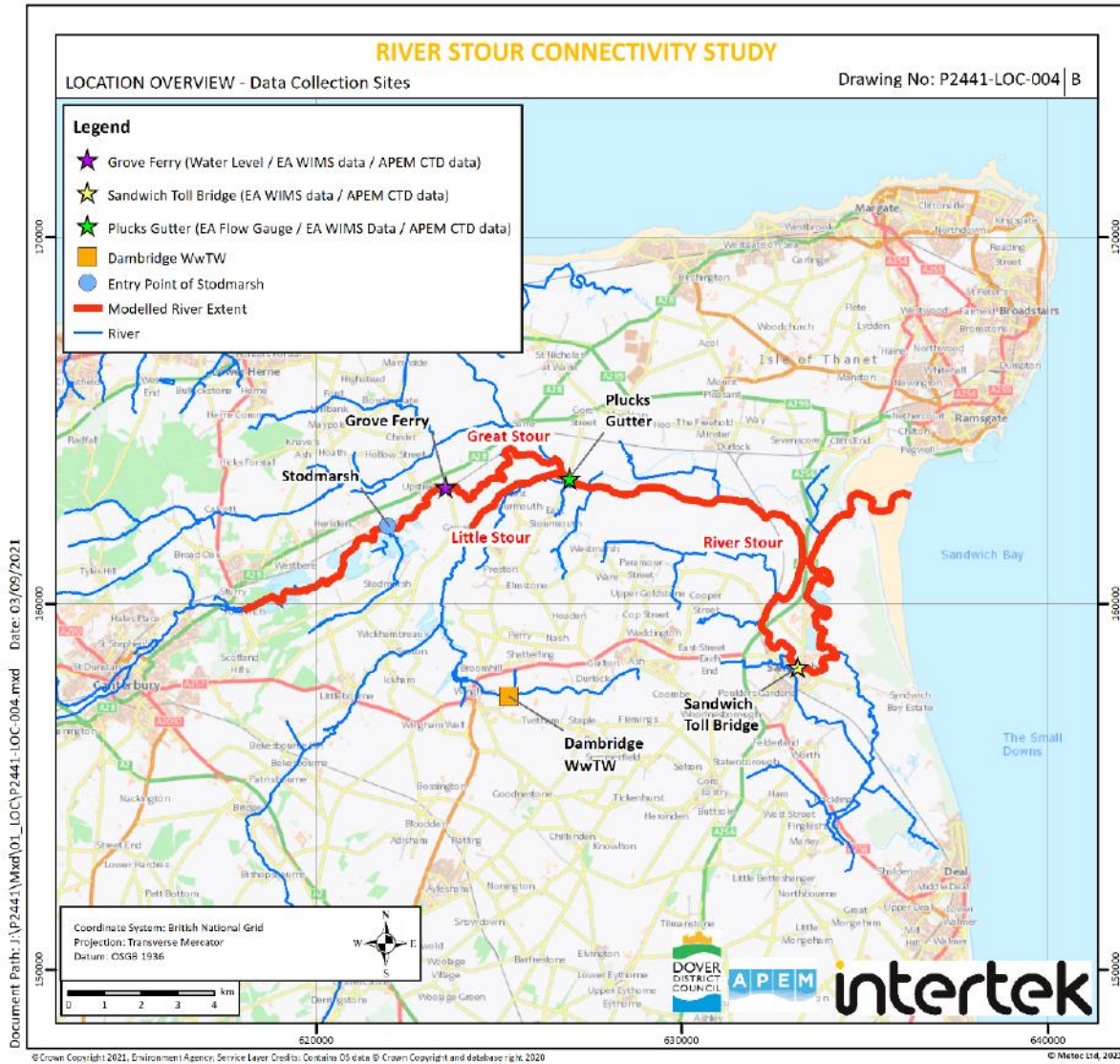
Figure 6. Calibration Locations
