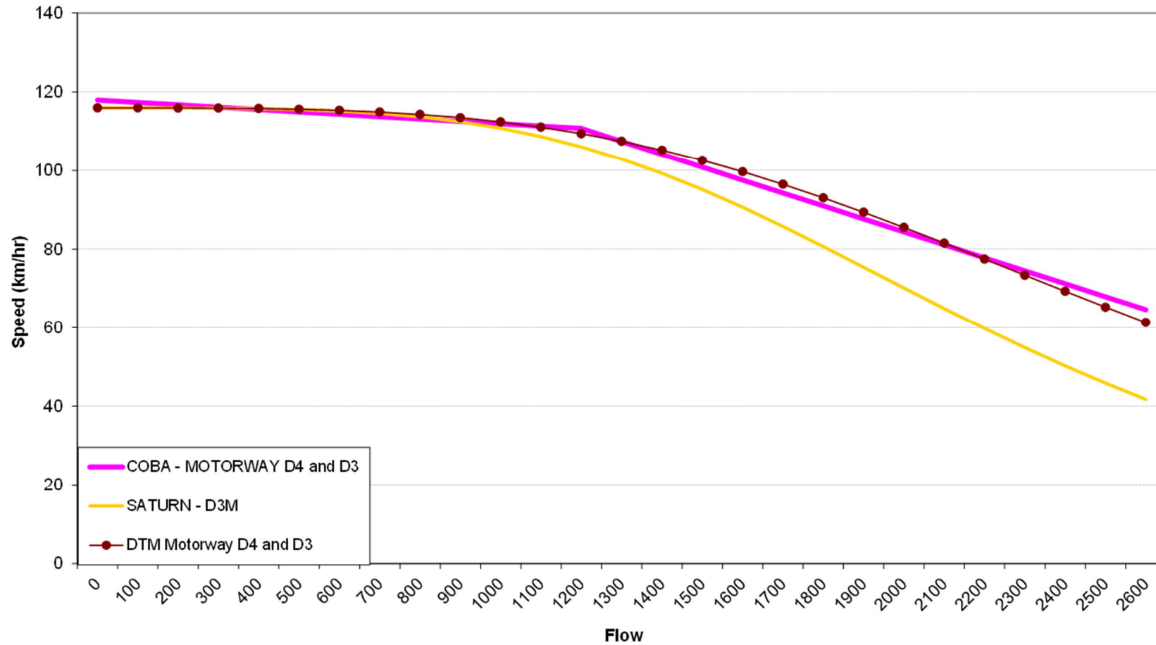
Motorway D4/3 Speedflow Curves
