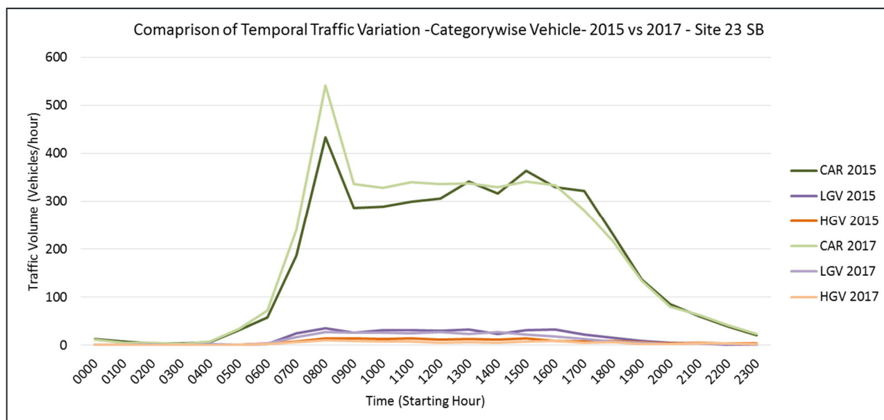
Figure 12: Comparison of Temporal Variation – by Vehicle Types – 2015 vs 2017 – Honeywood Parkway Southbound
